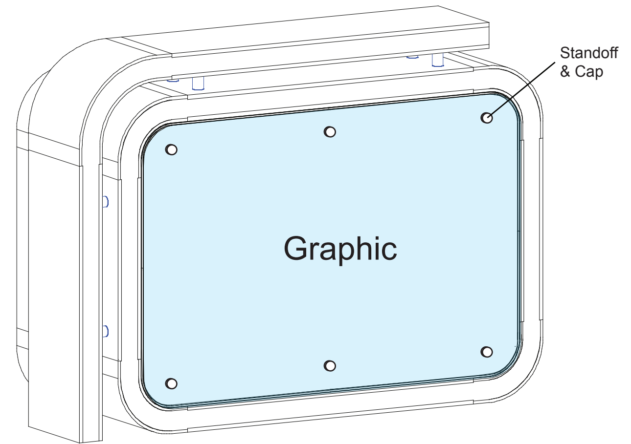
Completed Assembly
